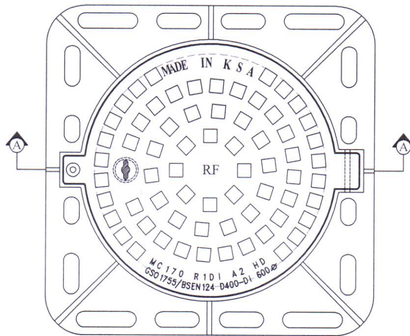
PLAN
